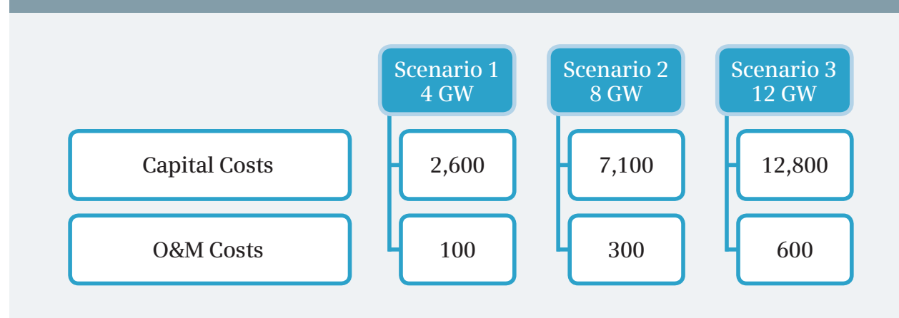
FIGURE 14: GRID COSTS IN € MILLIONS
