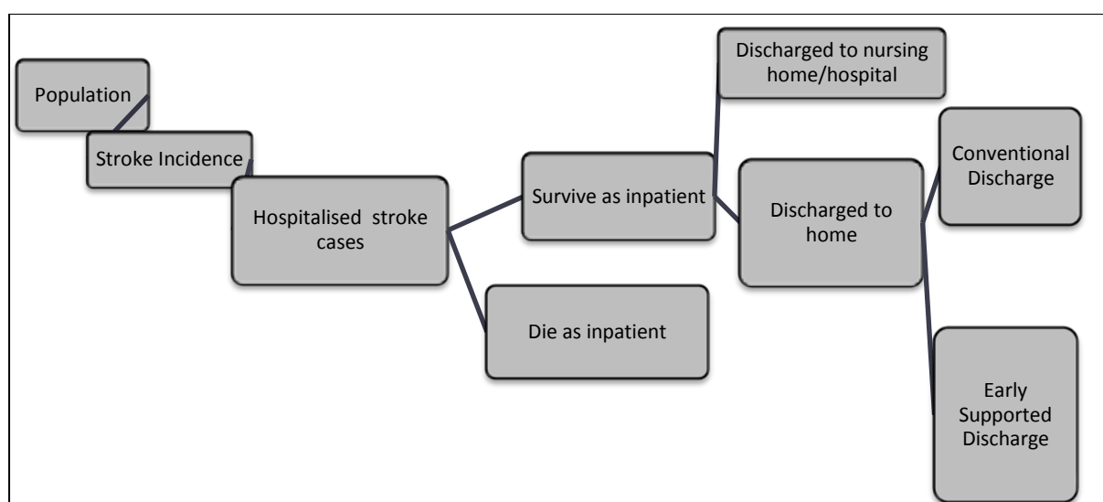
FIGURE 2 Decision-Tree Model
