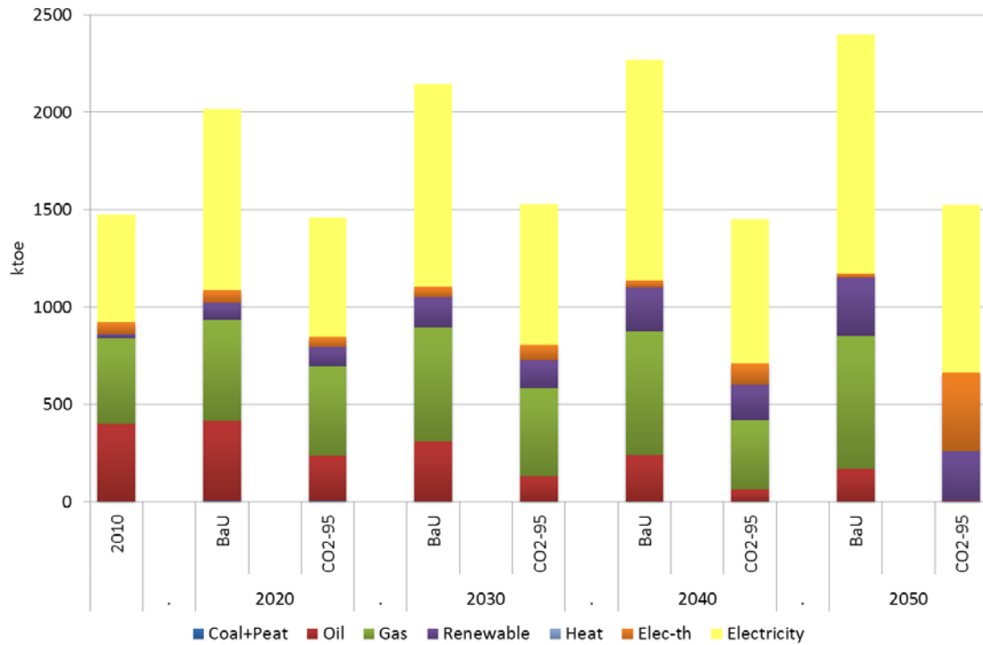
FIGURE 4-15-ENERGY CONSUMPTION IN THE SERVICES SECTOR FOR BAU AND 95% EMISSIONS REDUCTION SCENARIOS BY FUEL TYPE
