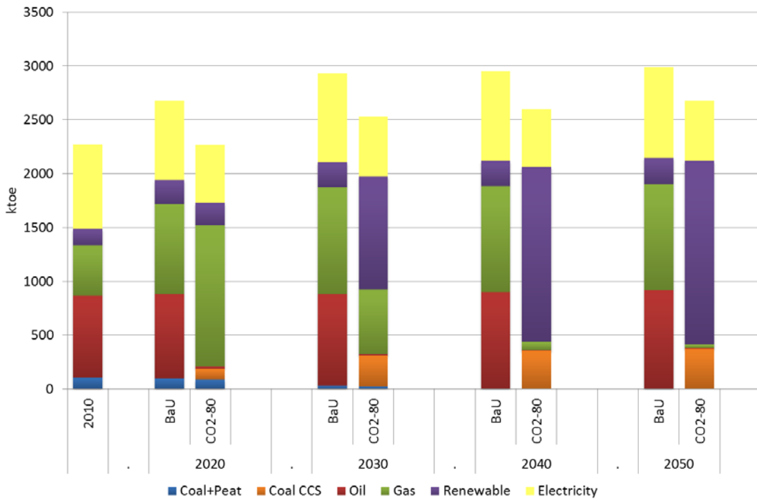
FIGURE 2-19: ENERGY COMSUMPTION IN THE INDUSTRIAL SECTOR FOR BAU AND CO2-80 SCENARIOS BY FUEL TYPE
