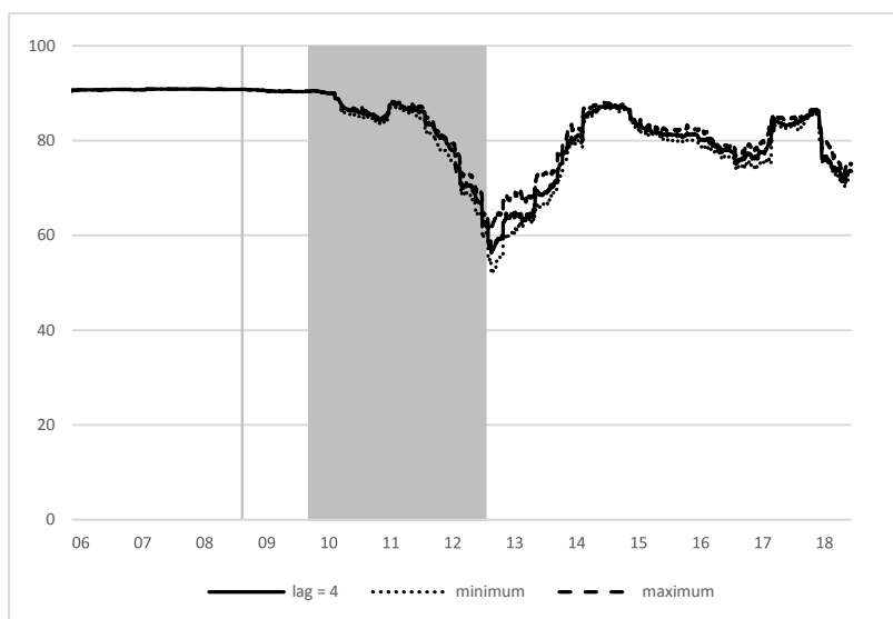
Figure 9a. Sensitivity of TSI to chosen lag length
